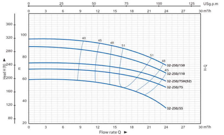
PERFORMANCE CHART AT n=2900RPM
