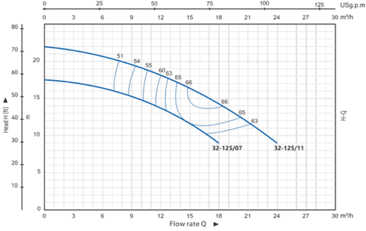
PERFORMANCE CHART AT n=2900RPM
