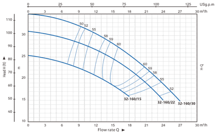
PERFORMANCE CHART AT n=2900RPM
